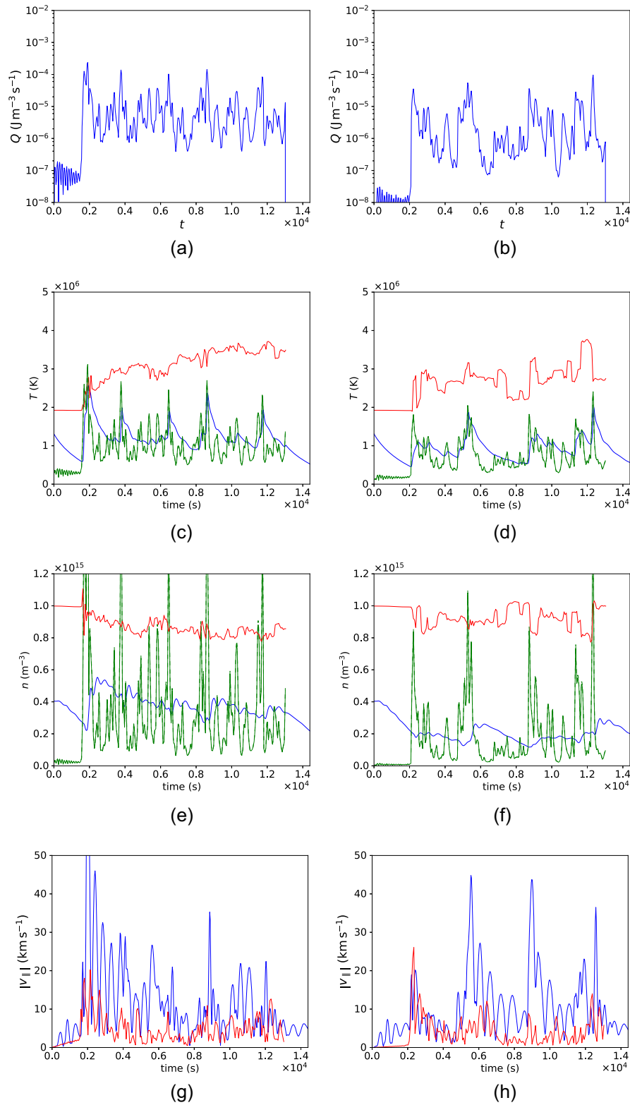
Figure 3. Averages of heating (top row), temperature ( T , second row), number density ( n , third row), and parallel velocity ( |v_{||}| , bottom row), for field lines (ii) (left column) and (v) (right). For the temperature, density, and velocity, coronal averages are taken over the half of the field line lying around the loop apex, and shown in blue. For velocity, the absolute value of field-aligned velocity is averaged. Red curves represent the results from the 3D model, green values obtained by inserting the average heating into the scaling laws of Martens (2010).
